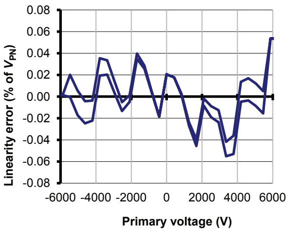
Figure 13: Typical linearity error at 25 °C
